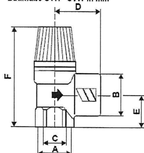
Baumaße SVH - SVW in mm
